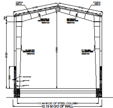
PORTAL FRAME AT 2
