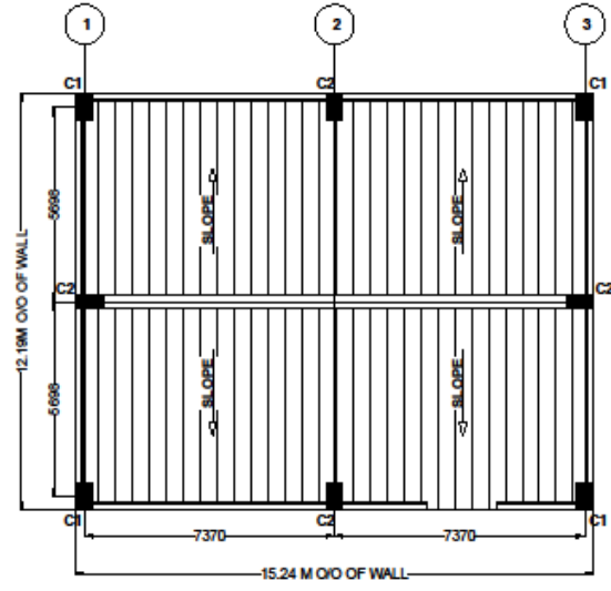
ROOF PLAN
