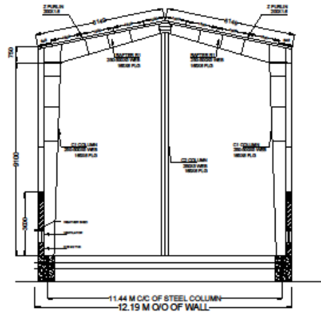
PORTAL FRAME AT 1 & 3
