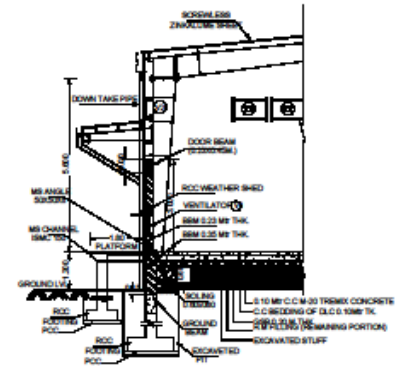
DETAILS OF FOOTING COLUMN BEAM PLATFORM TRUSS
